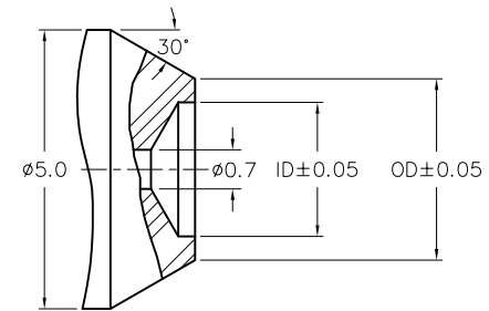
DESIGN "C"(WITH SECTION) SCALE 10:1
