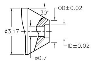
DESIGN "B"(WITH SECTION) SCALE 10:1
